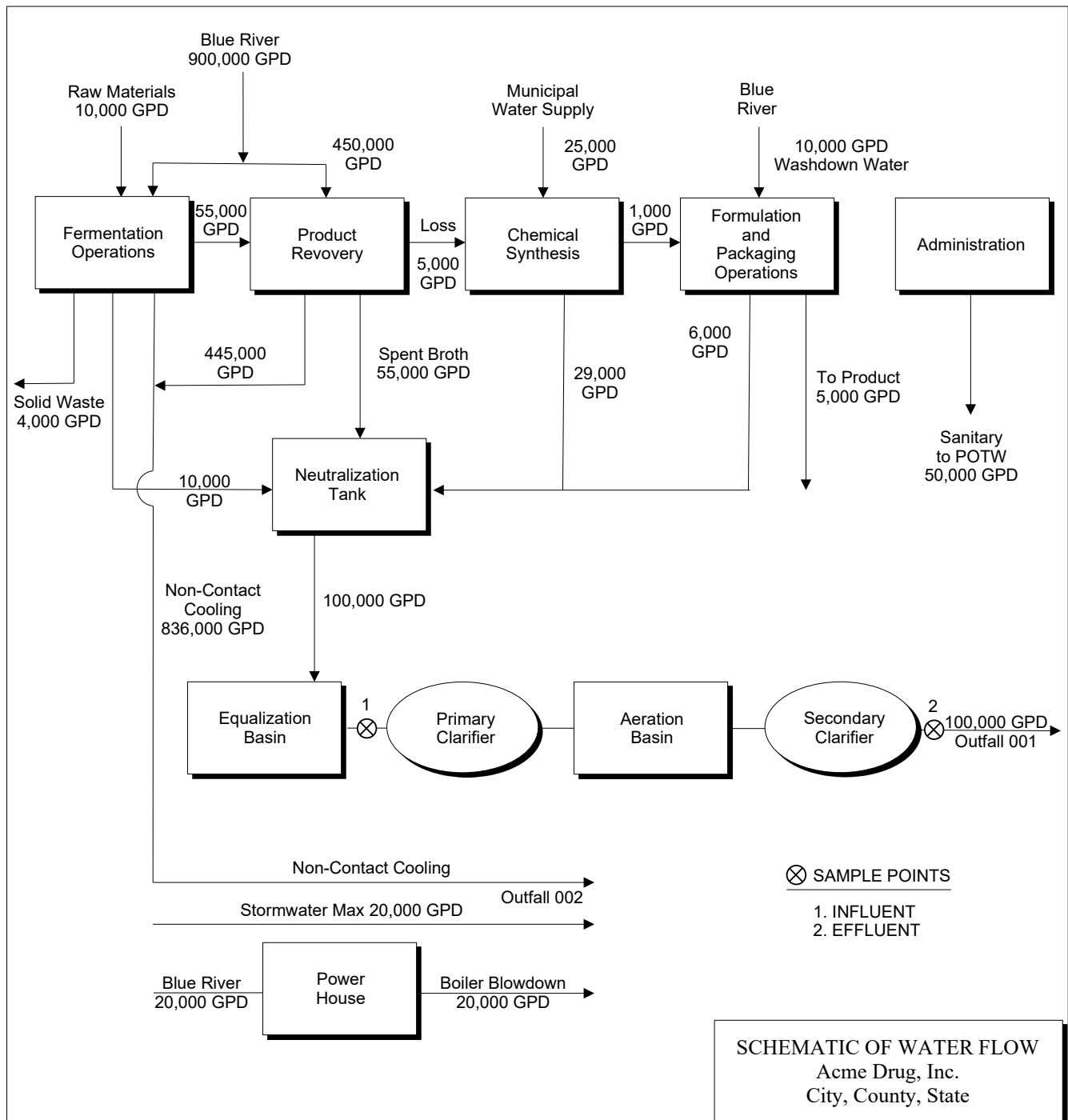
Figure 1. SCHEMATIC FLOW DIAGRAM
